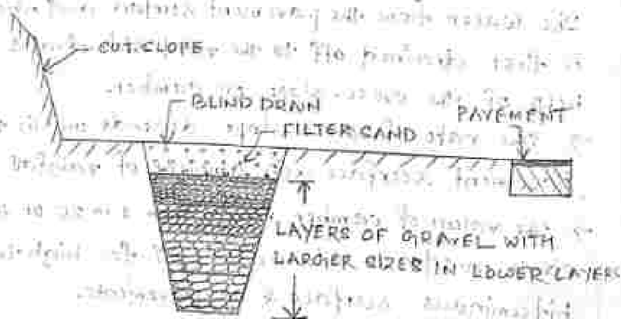
(DRAINAGE TRENCH FILLED WITH FILTER MATERIAL)
